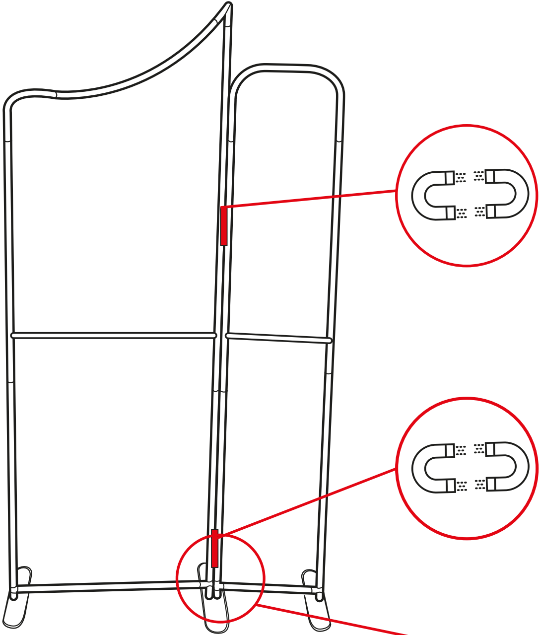
824 Slope 1 Frame and 420 Straight Frame
