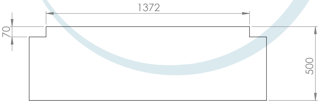
Cutting the last sheet of roof covering
