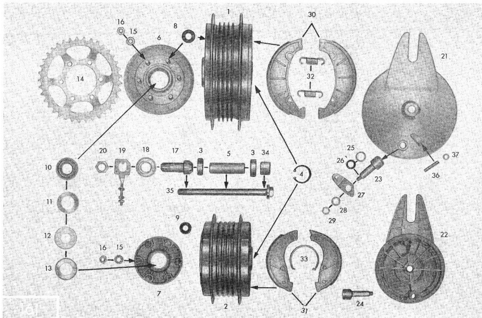
Tafel 24/3 Hinteres Laufrad, Hinterradnabe Table 24/3 Rear wheel, rear wheel hub Planche 24/3 Roue AR, moyeu de roue AR
