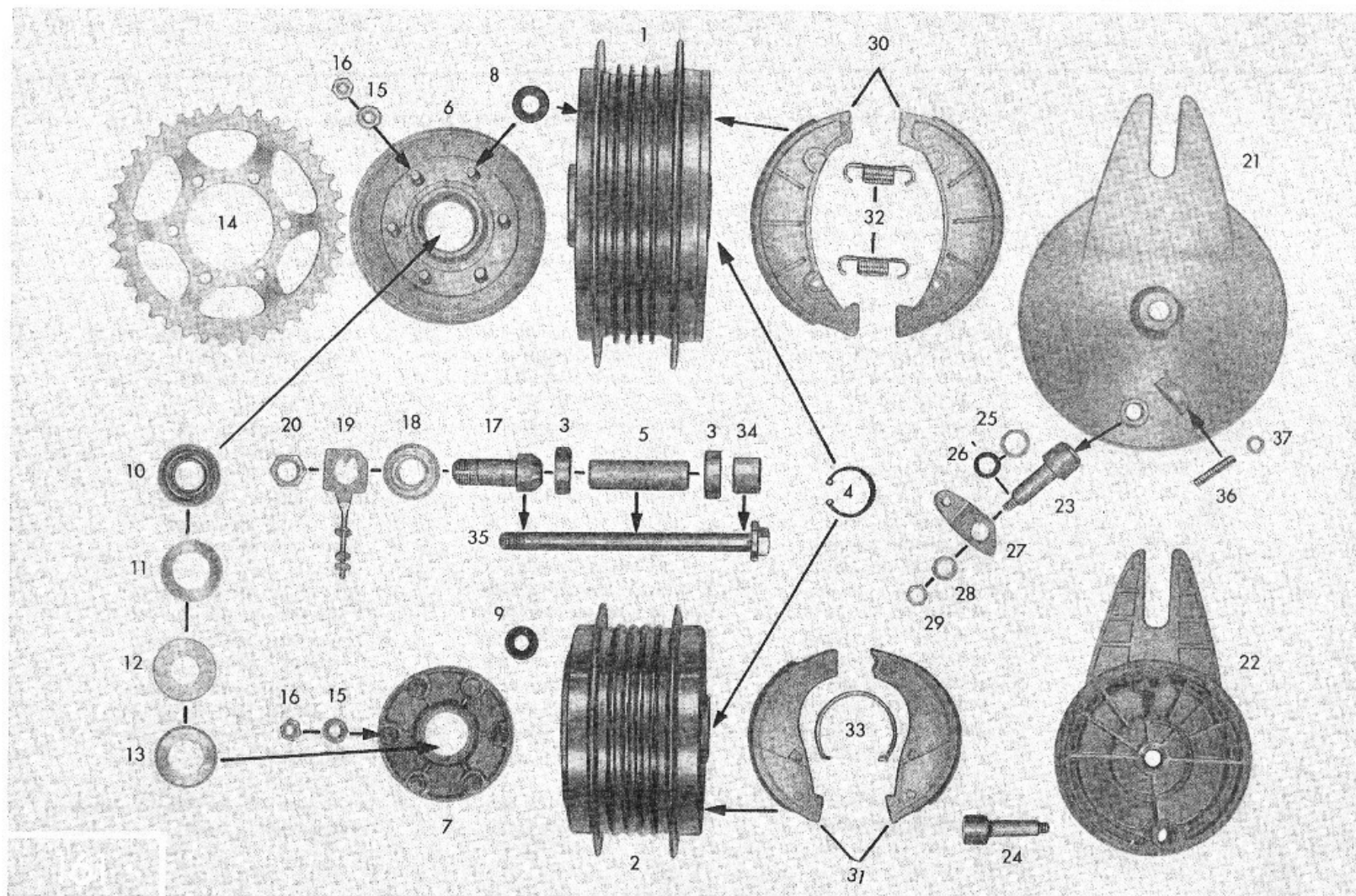
Tafel 24/1 Hinteres Laufrad, Hinterradnabe Table 24/1 Rear wheel, rear wheel hub Planche 24/1 Roue AR, moyeu de roue AR
