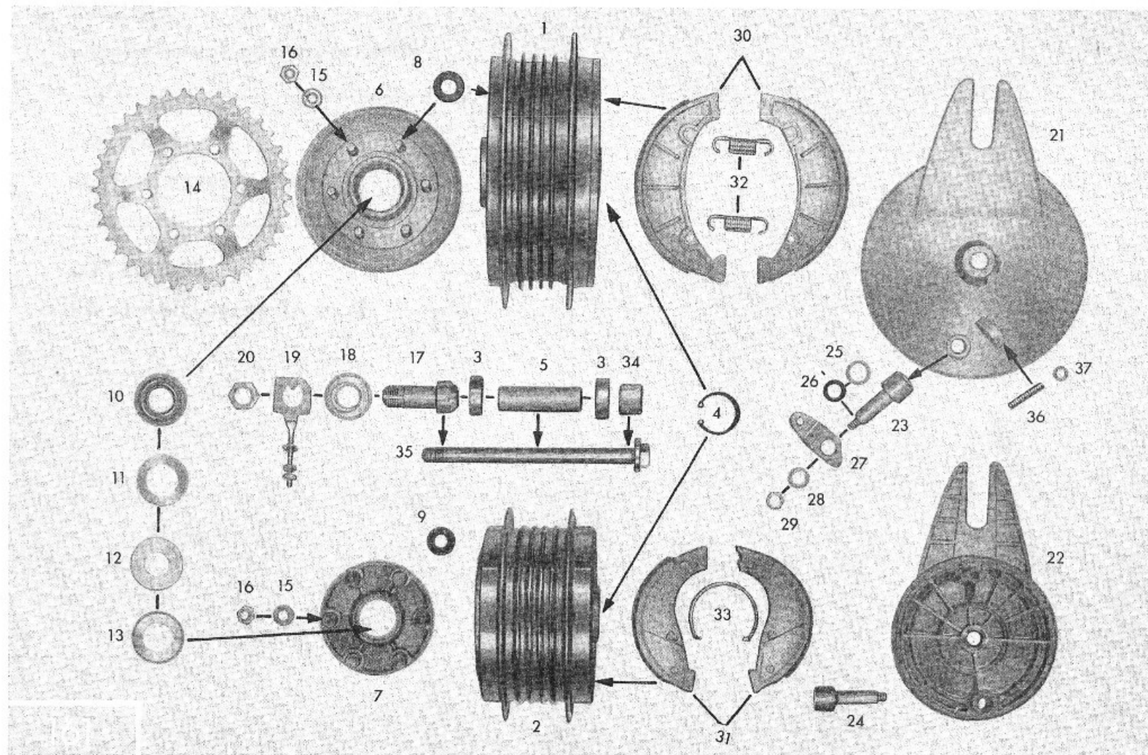
Tafel 24/2 Hinteres Laufrad, Hinterradnabe Table 24/2 Rear wheel, rear wheel hub Planche 24/2 Roue AR, moyeu de roue AR
