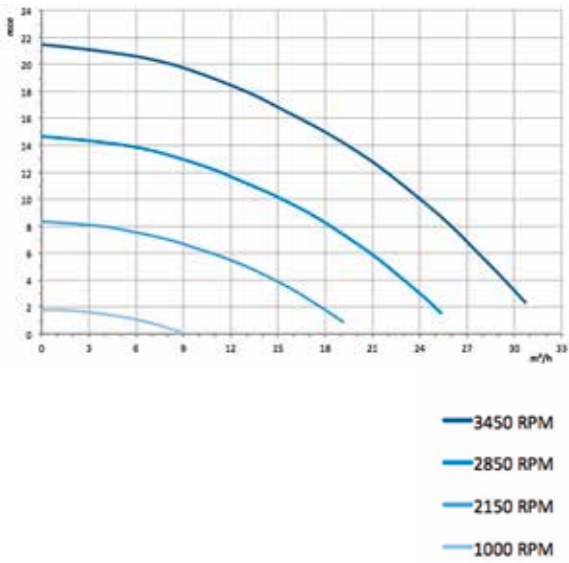
FLOPRO VS/FLOPRO VS AUT PUMPKAPACITET
