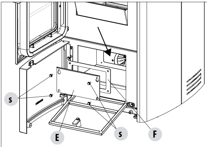
CLEANING THE LOWER COM- PARTMENT
