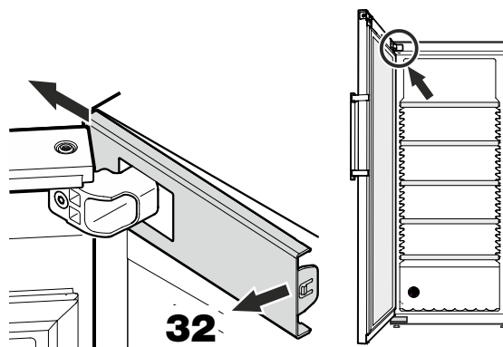
32. Release cover on the inside and slide to the outside.
