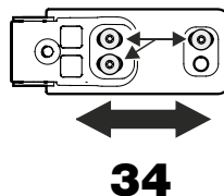
34. Undo screws and slide hinge bracket to the right or left.
