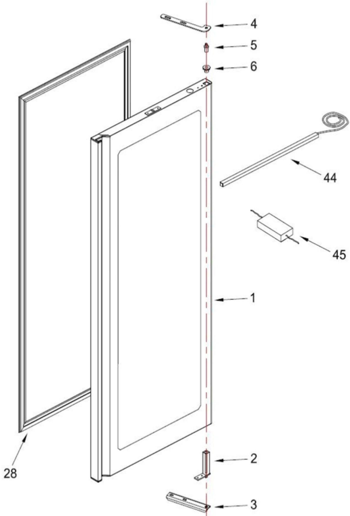
VERTICAL REFRIGERATORS - GLASS DOOR DETAIL
