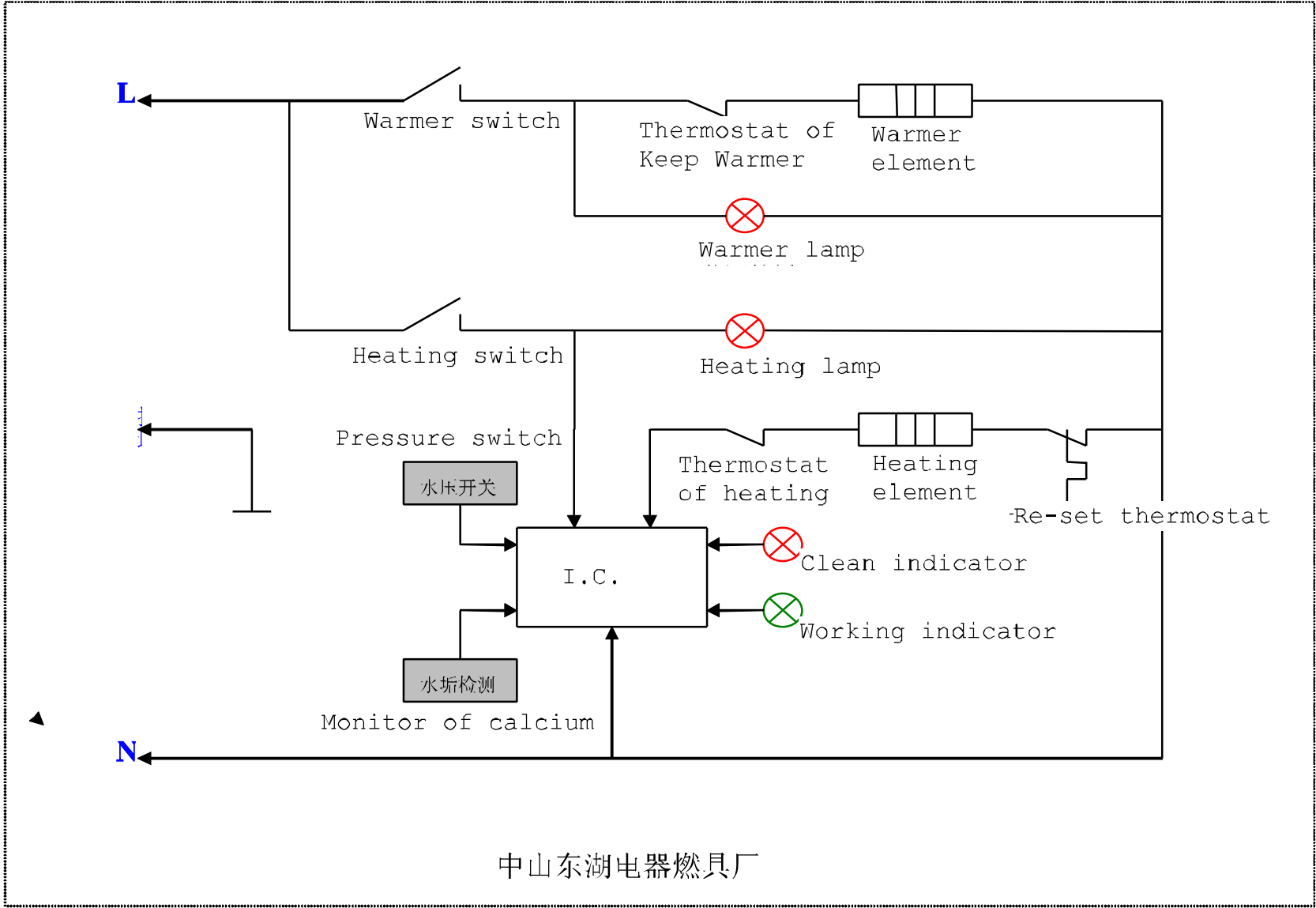
ND1002D |Circuit Diagram of Coffee machine
