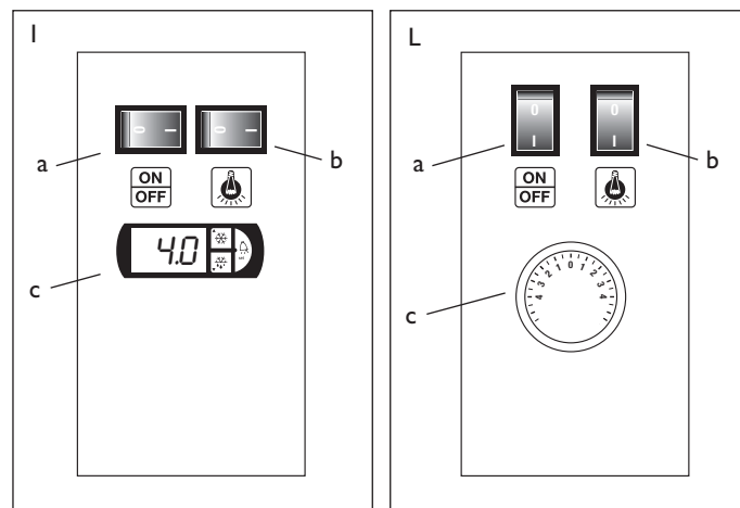
CONTROL DEVICES – MODELS VR 2000 AND VR 2005 (Fig. I)
