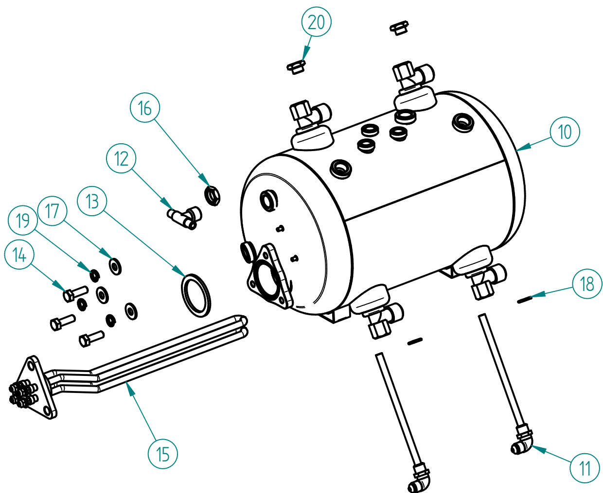
1 - 7.0.000.0533 - CALDEIRA 2GR 11 LT C/ ACESS. 1 - 2 GROUP 11 LT BOILER W/ ACCESS.
