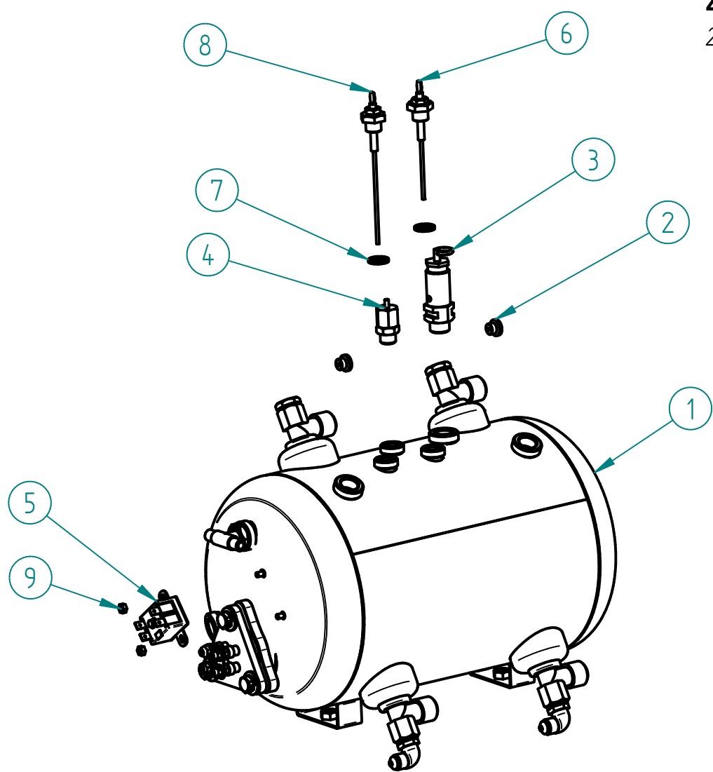
1 - 7.0.000.0533 - CALDEIRA 2GR 11 LT C/ ACESS. 1 - 2 GROUP 11 LT BOILER W/ ACCESS.
