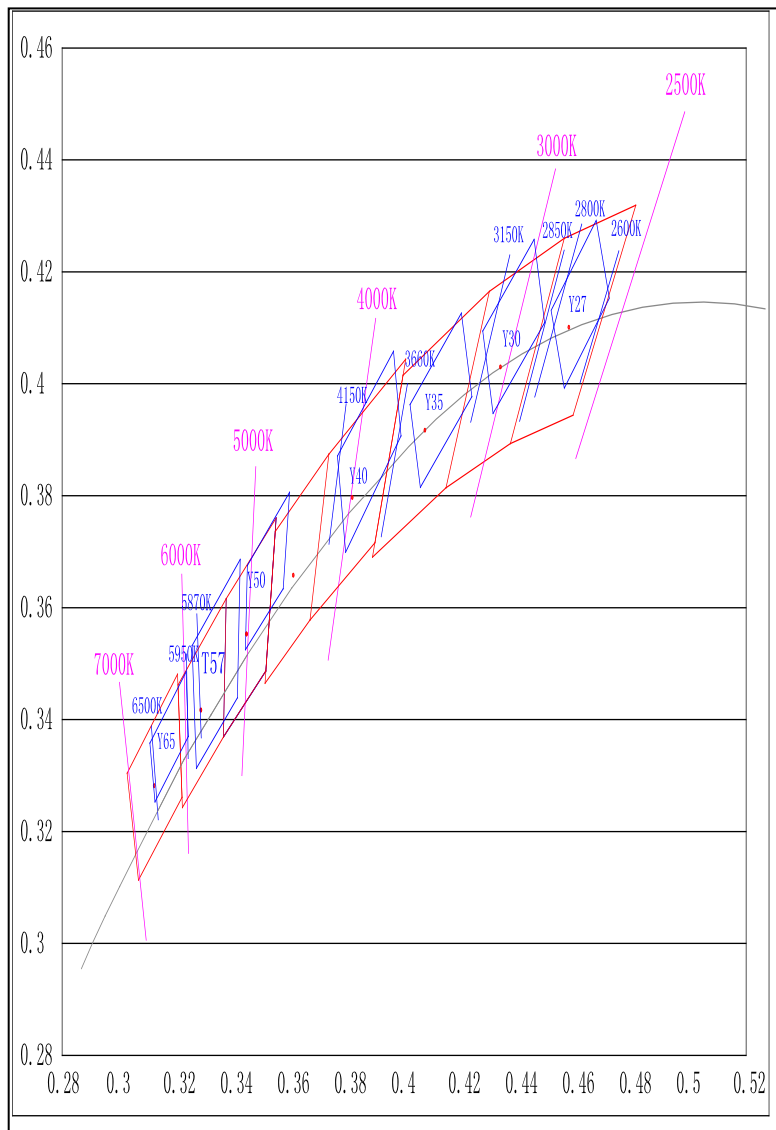
Correlated color temperature bin definitions for 2835R Series at rated current, Ta =25°C
