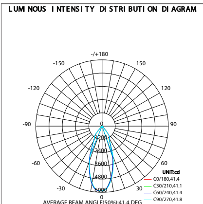
Downlight Forza V2 8719157067423 3000K Black
