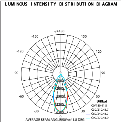
Downlight Forza V2 8719157067416 3000K White
