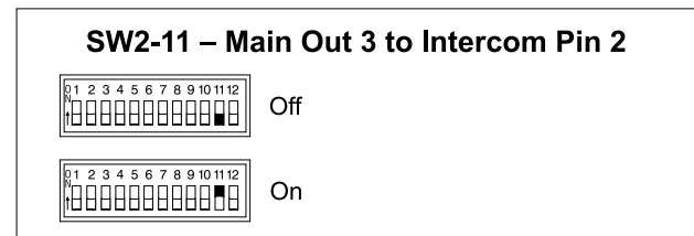
Figure 9. Main output 3 to intercom pin 2 settings
