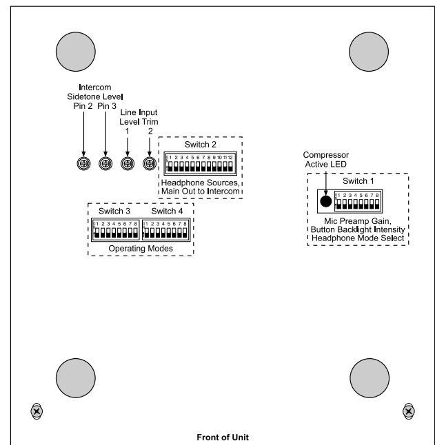
Figure 4. Bottom view of Model 240 showing configuration switches, trim pots, and compressor active LED
