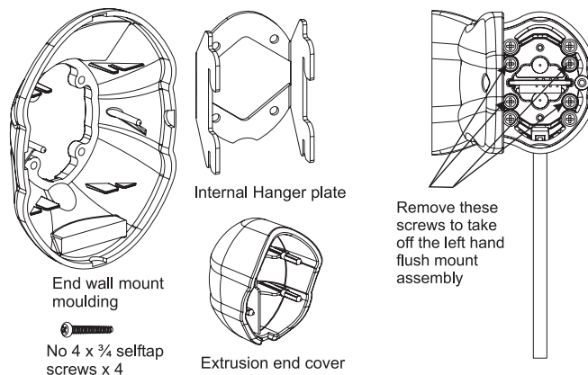
Fig 5-2: Kit Components Used for the Conversion
