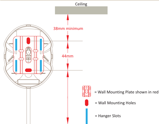
Fig 2-2: End Mounting Requirements
