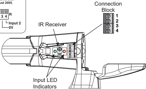
Fig 2-6: Mode Settings & Connection Block
