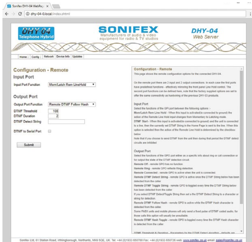
Figure 6-7: Remote Port Configuration – settings of remote port and DTMF detection – accessed via Config Menu drop-down.
