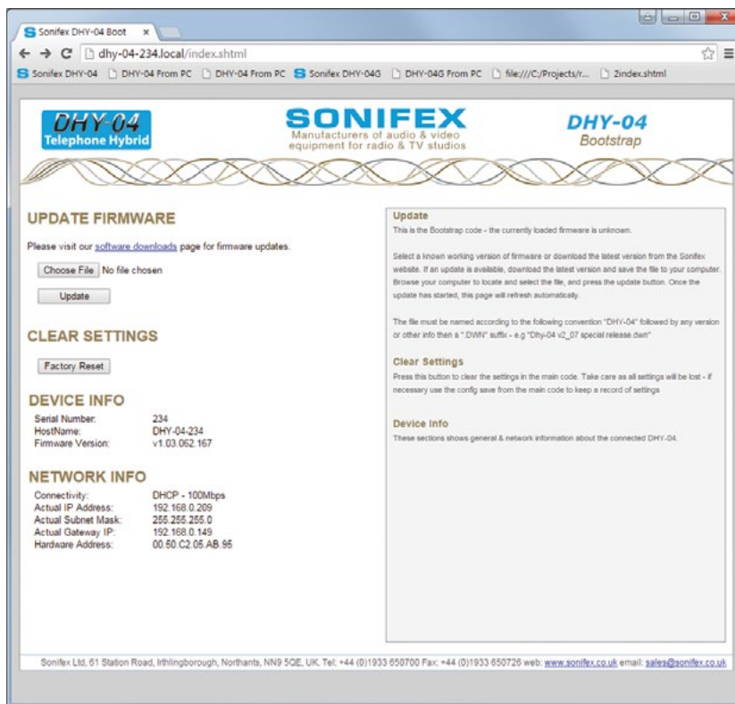
Figure 6-14: Bootstrap Page.
