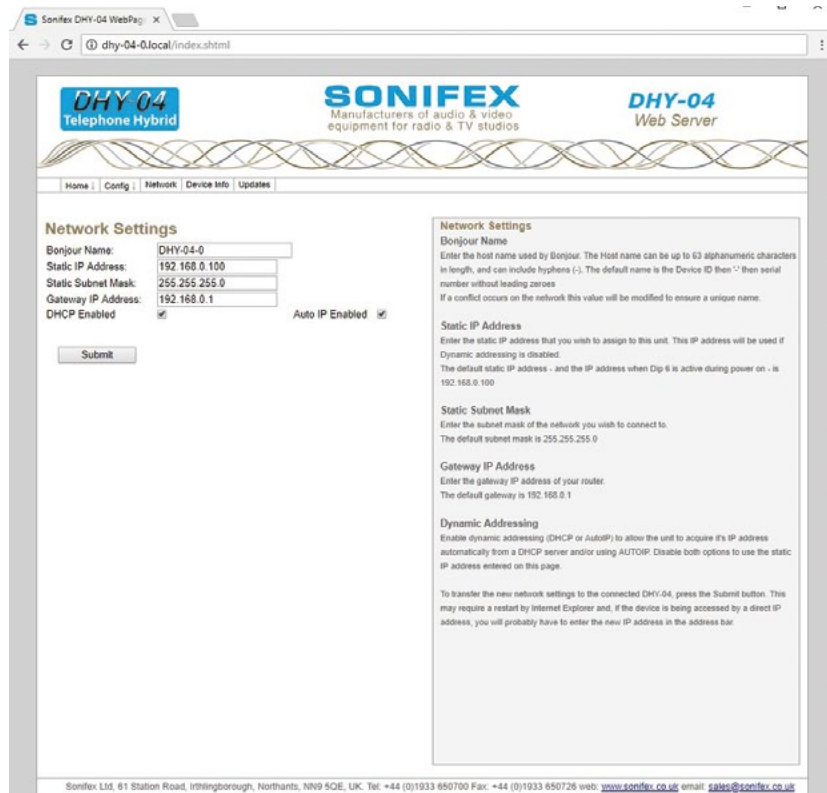
Figure 6-10: Network Page – settings for network interface.
