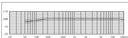
Frequency response curve CCM 41
