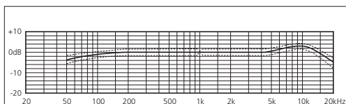
Frequency response curve CCM 4V
