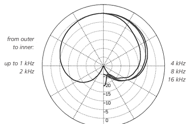
Polar diagram CCM 4P, CCM 4XP
