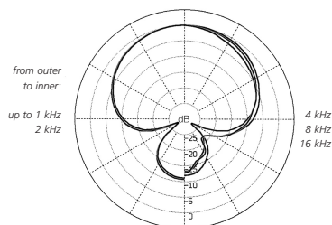
Polar diagram CCM 41
