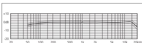
Frequency response curve CCM 41V
