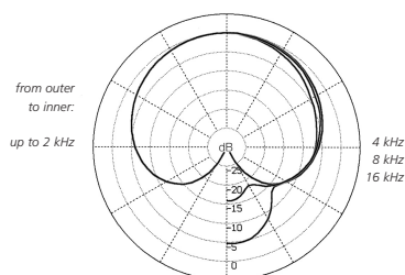
Polar diagram CCM 4V
