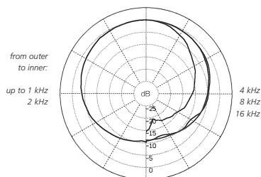
Polar diagram CCM 21, -21H
