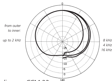
Polar diagram CCM 22
