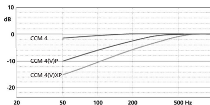
Low-frequency response curves of the two microphone types (P and XP) compared to the standard CCM 4 (measured at a 60 cm equivalent distance).
