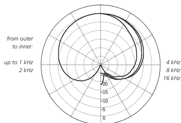
Polar diagram CCM 4
