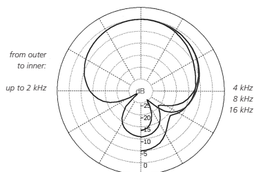
Polar diagram CCM 41V
