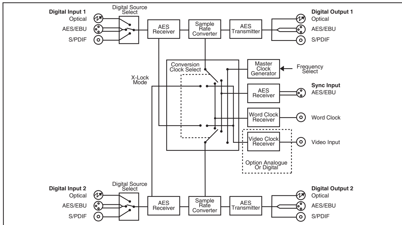
Fig 4-4: RB-SC2 System Block Diagram
