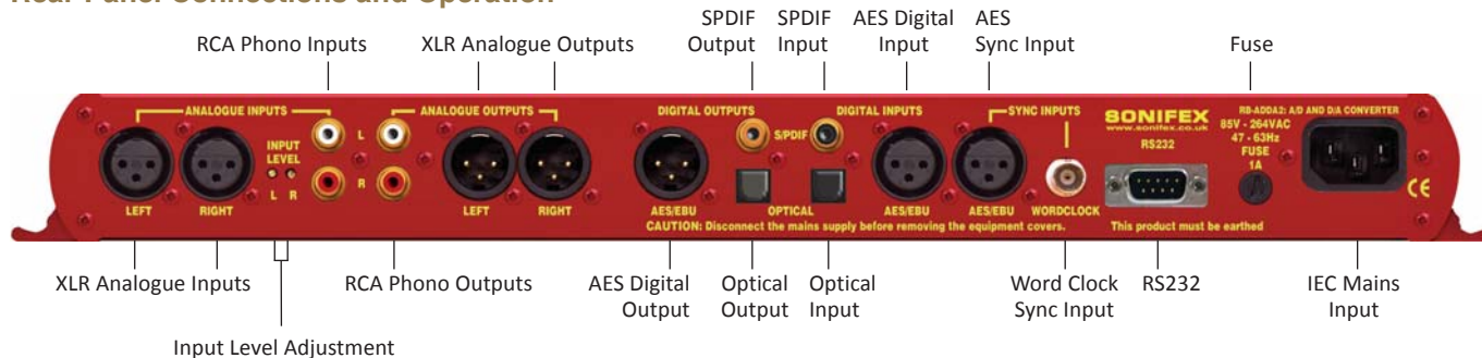
Fig 2-9: RB-ADDA2 Rear Panel
