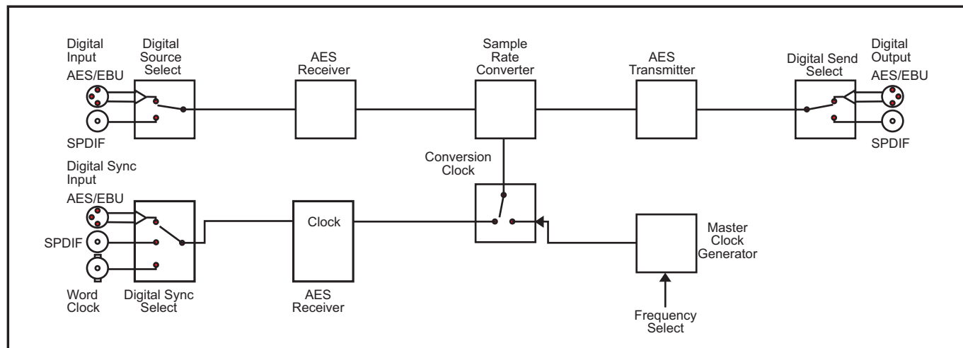
Fig 3-2: RB-SC1 System Block Diagram
