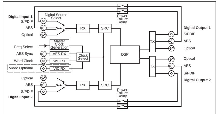
Fig 11-2: RB-DD4 Block Diagram
