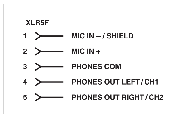
Figure 2. Headset connection pinout chart
