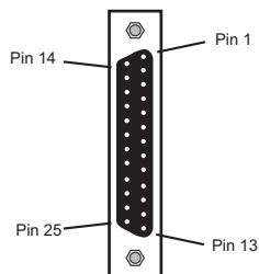
Fig 2-8 : 25 Pin D-Type Connectors.
