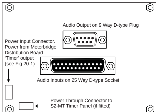
Fig 20-10b : S2-M6SS Diagram.
