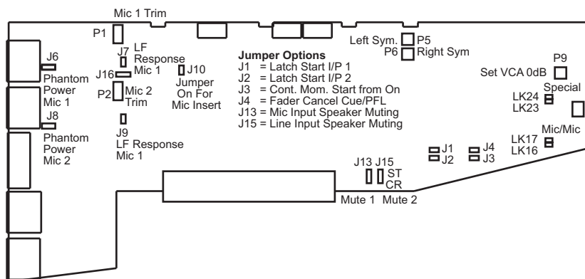
Fig 6-1 : S2 Mic/Mic Input Board Layout.
