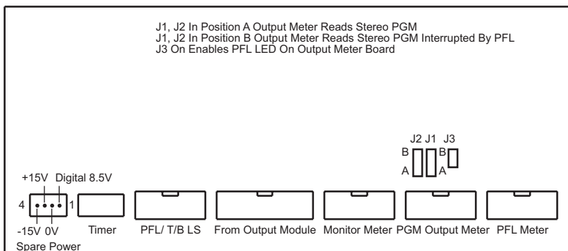
Fig 20-1 : Meterbridge Distribution Board Layout.
