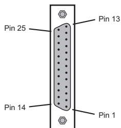
25 Pin D-Type Socket used for Remotes
