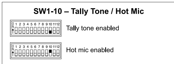
Figure 9. Tally tone/hot mic out switch settings
