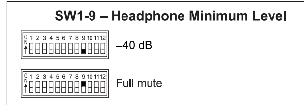
Figure 8. Headphone minimum level switch settings
