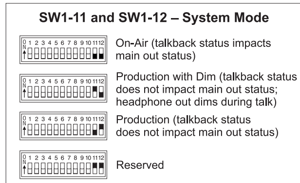
Figure 10. System mode settings
