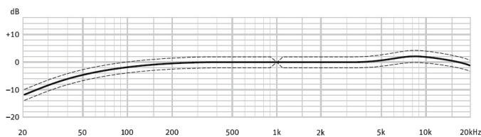
FREQUENCY RESPONSE
