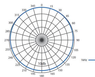
POLAR PATTERN @ 1kHz
