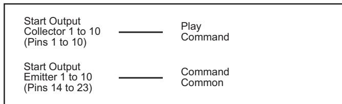
Fig 2-7: Connection Example
