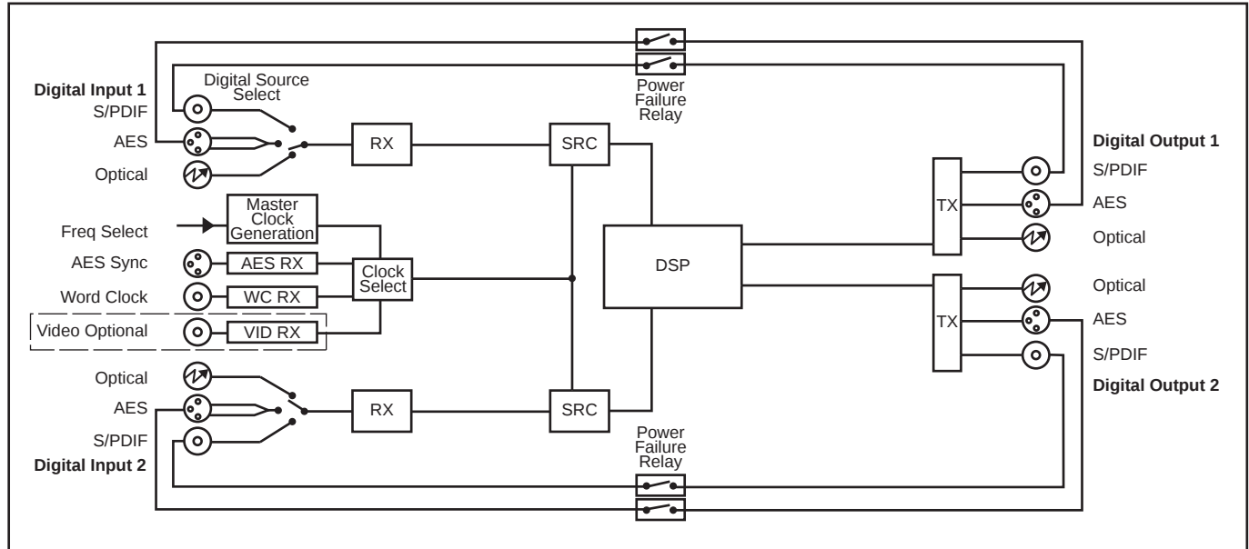
Fig 4-2: RB-DMX4 System Block Diagram
