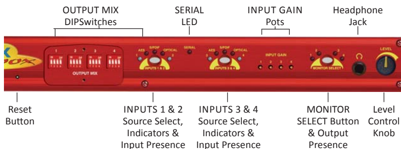
Fig 4-3: RB-DMX4 Front Panel Controls and Indicators
