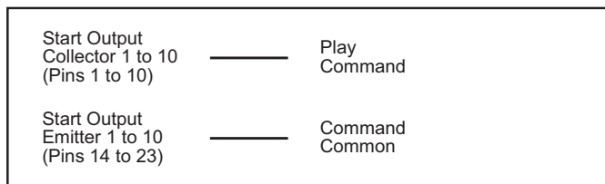
Fig 1-7: Connection Example
