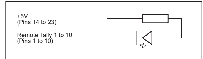
Fig 1-11: Connection Example
