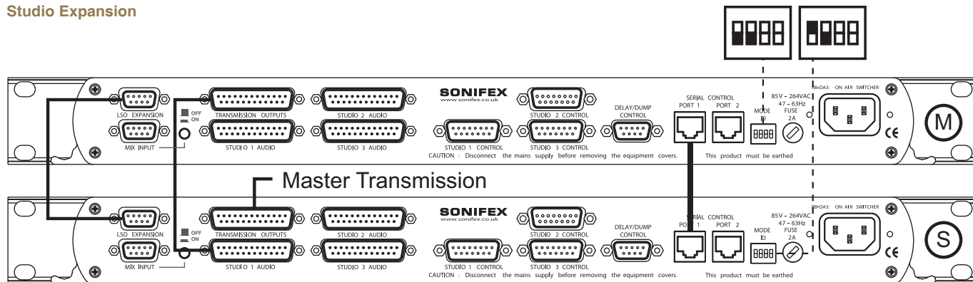
Fig 6-6: RB-OA3 Studio Expansion Diagram
