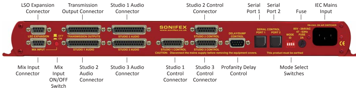
Fig 6-3: RB-OA3 Rear Panel
