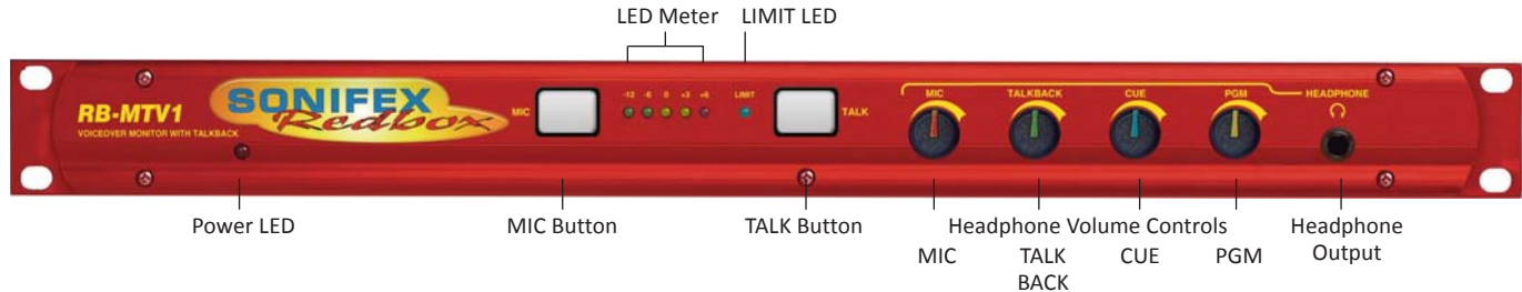
Fig 10-1: RB-MTV1 Front Panel
