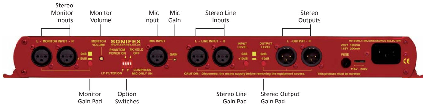
Fig 5-3: RB-SSML1 Rear Panel.
