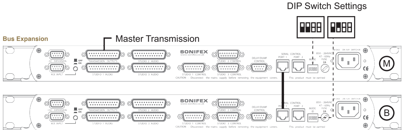
Fig 6-7: RB-OA3 Bus Expansion Diagram
