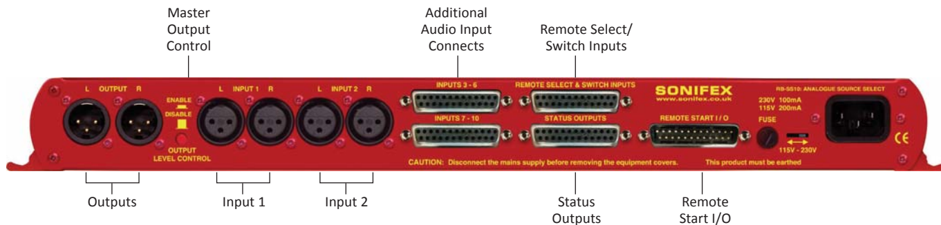
Fig 1-4: RB-SS10 Rear Panel
