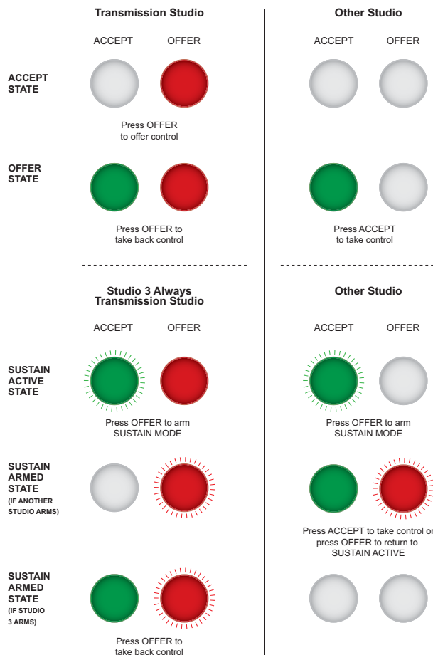
Fig 6-10: Offer & Accept Button Operation (Flashing is indicated by radial lines around a button)
