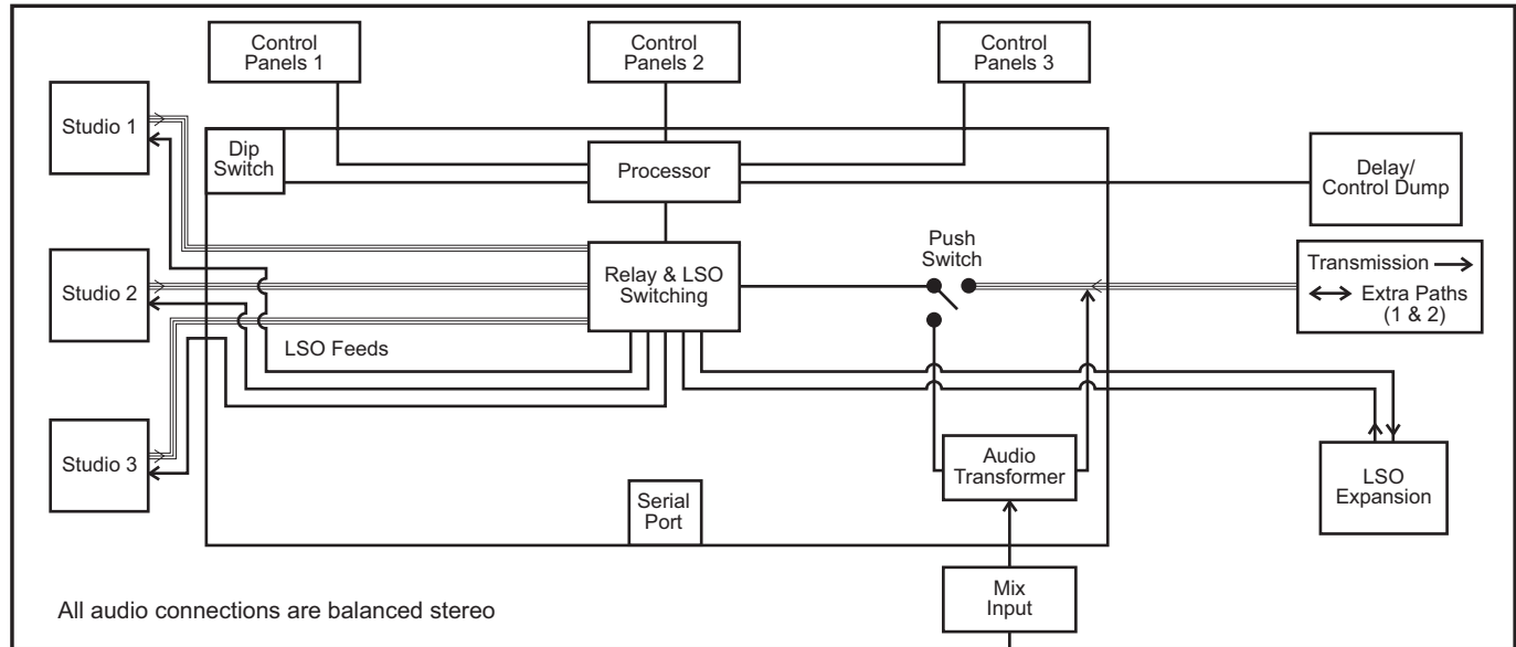
Fig 6-2: RB-OA3 System Block Diagram
