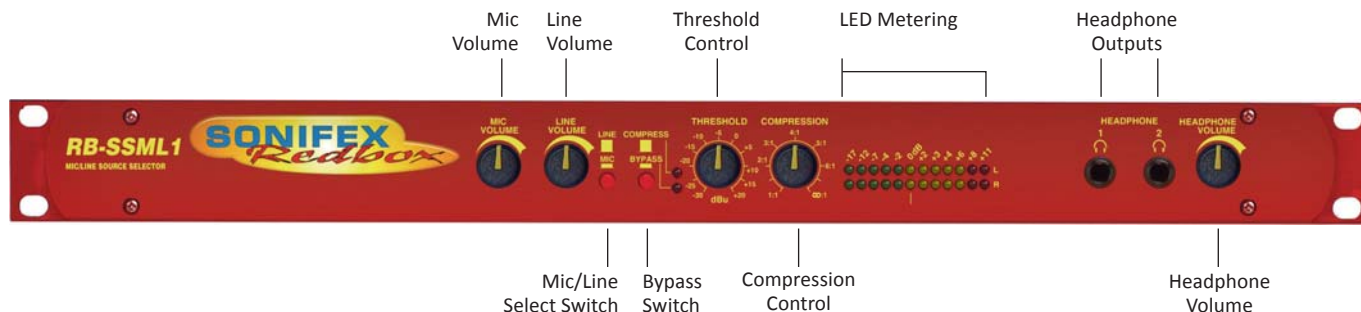
Fig 5-1: RB-SSML1 Front Panel
