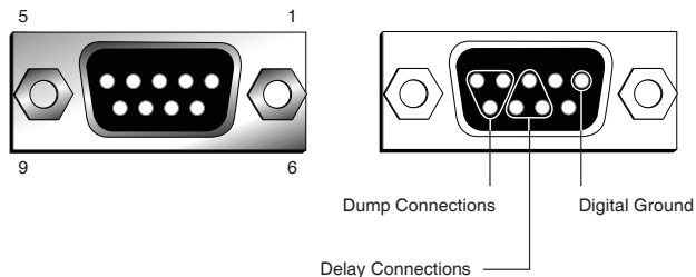
Fig 6-22: RB-OA3 Profanity Delay Control Connector Details
