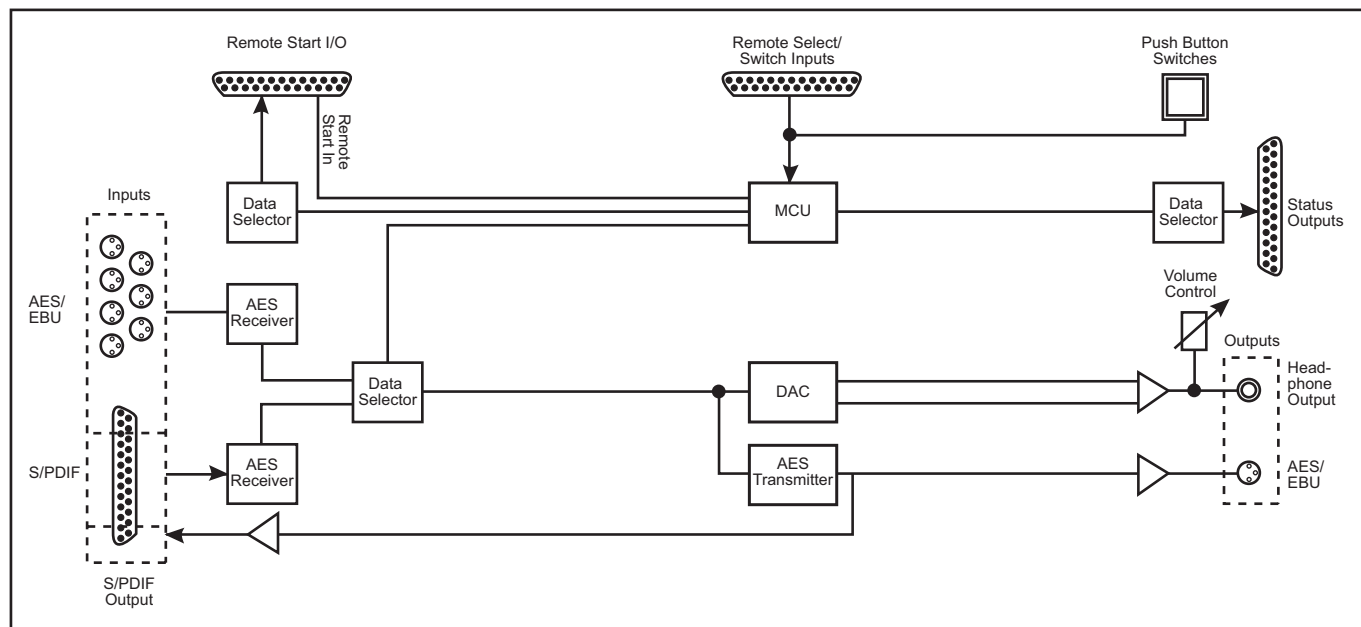
Fig 2-2: RB-DSS10 System Block Diagram
