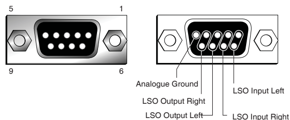
Fig 6-11: RB-OA3 LSO Expansion Connector Definitions
