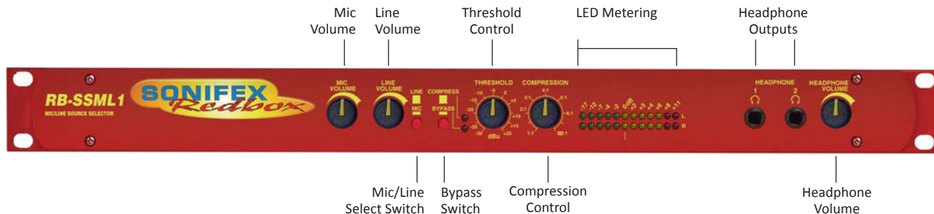
Fig 5-5: RB-SSML1 Front Panel
