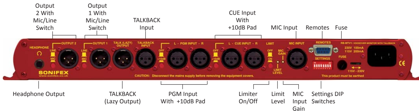
Fig 10-8: RB-MTV1 Rear Panel Connections
