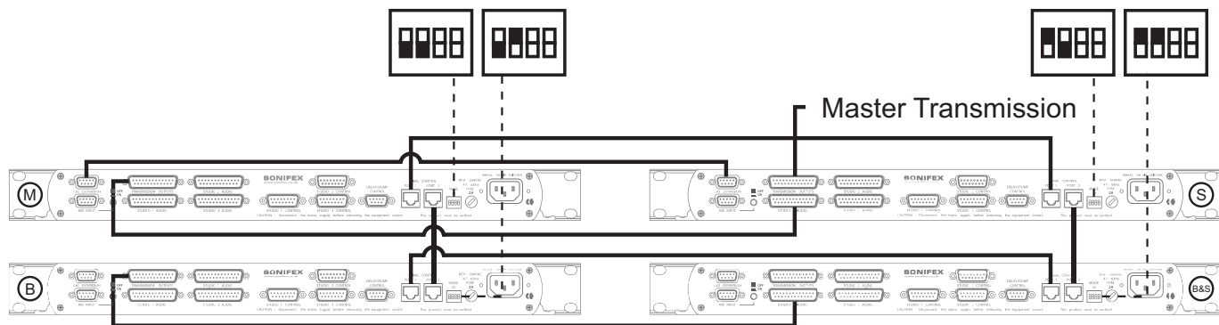
Fig 6-8: RB-OA3 Studio &amp; Bus Expansion Diagram
