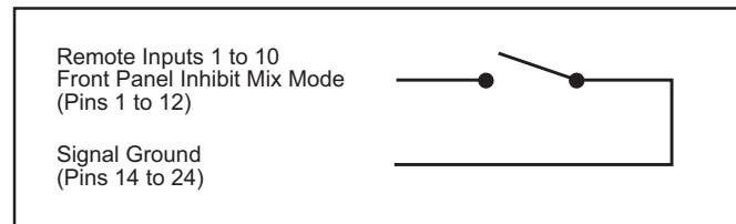
Fig 1-9: Connection Example
