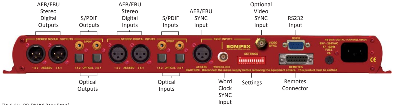
Fig 4-11: RB-DMX4 Rear Panel
