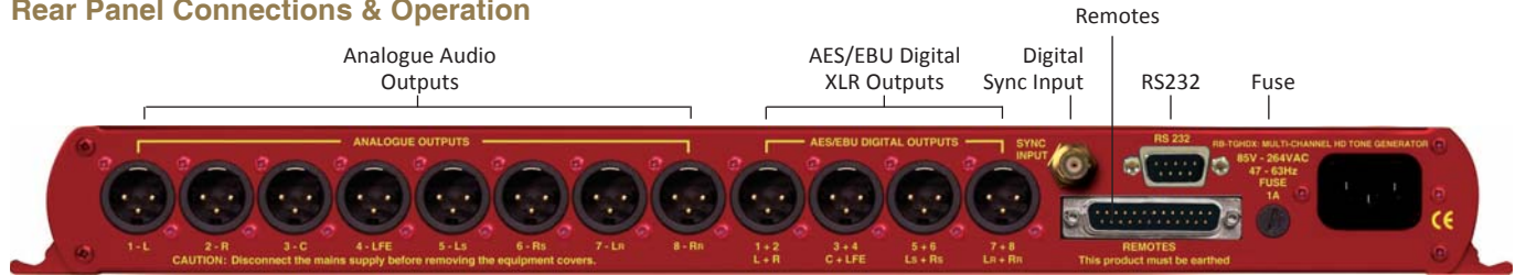
Fig 12-8: RB-TGHDX Rear Panel
