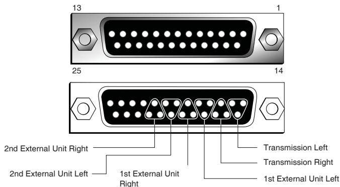
Fig 6-16: RB-OA3 Transmission Outputs Connector Details
