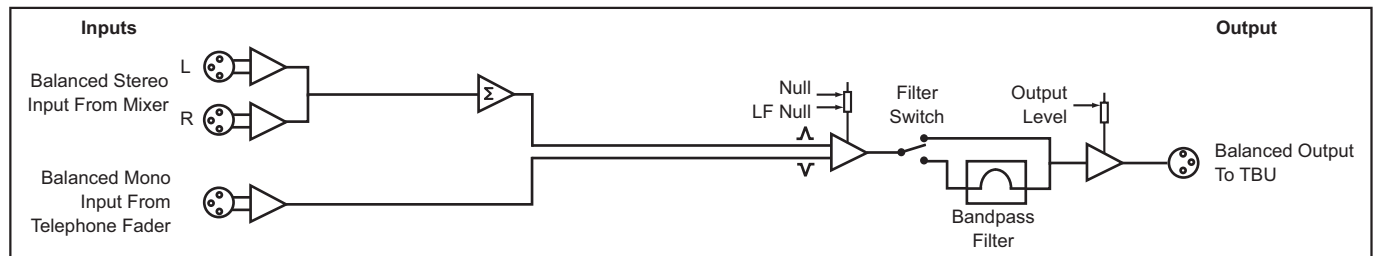
Fig 9-2: RB-MM1 System Block Diagram
