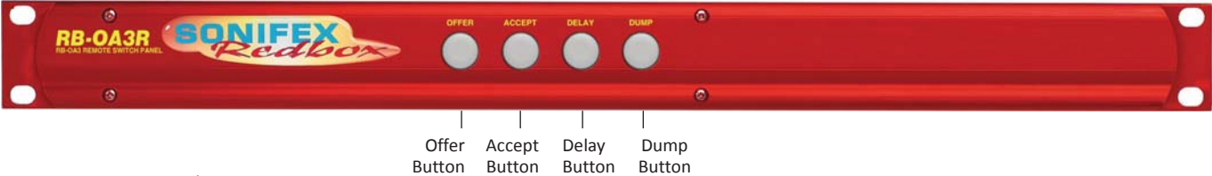
Fig 7-1: RB-OA3R Front Panel
