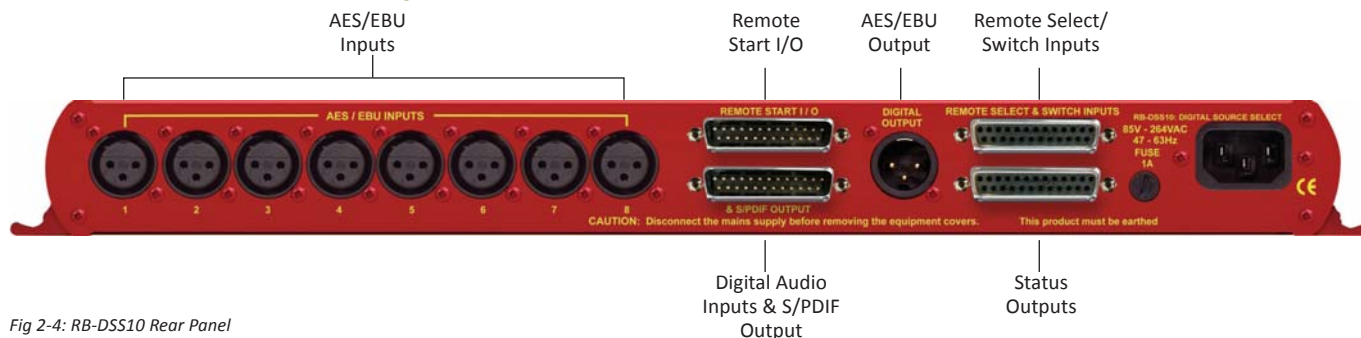
Fig 2-4: RB-DSS10 Rear Panel
