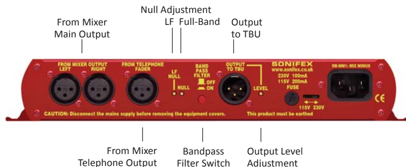
Fig 9-3: RB-MM1 Rear Panel.
