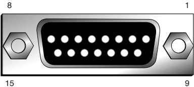
Fig 7-5: RB-OA3R Pin Out Positions
