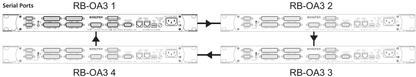
Fig 6-9: RB-OA3 Multiple RB-OA3 Expansion Diagram
