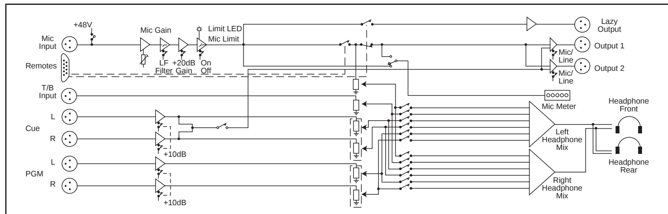
Fig 10-2: RB-MTV1 Block Diagram
