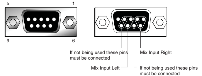
Fig 6-14: RB-OA3 Mix Input Connector Details
