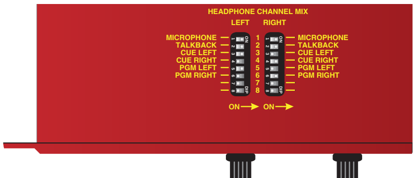
Fig 10-9: Underside of RB-MTV1 Showing Headphone Channel Mix DIPswitches
