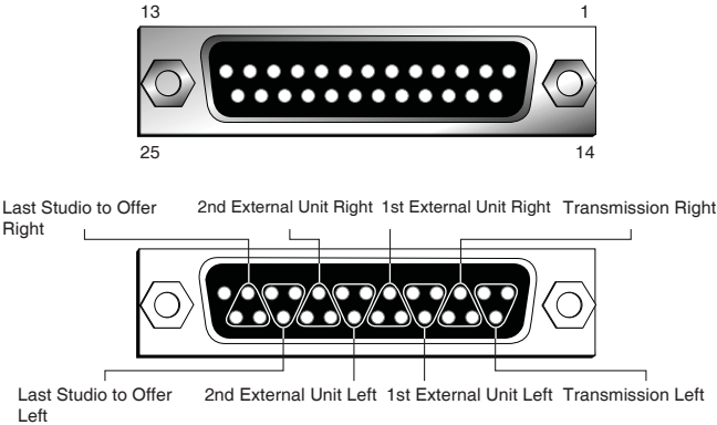
Fig 6-18: RB-OA3 Studio 1-3 Audio Connector Details
