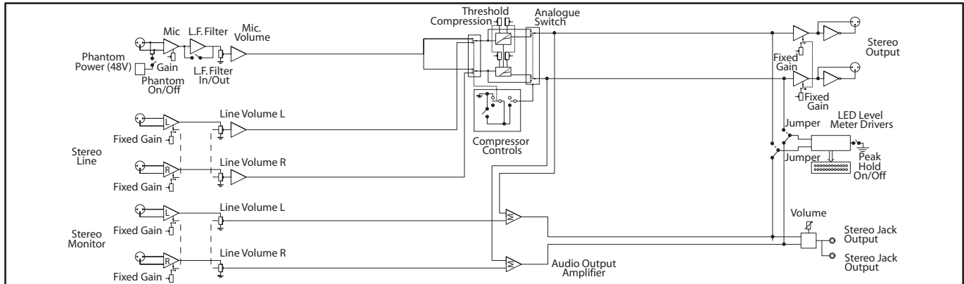
Fig 5-2: RB-SSML1 Block Diagram
