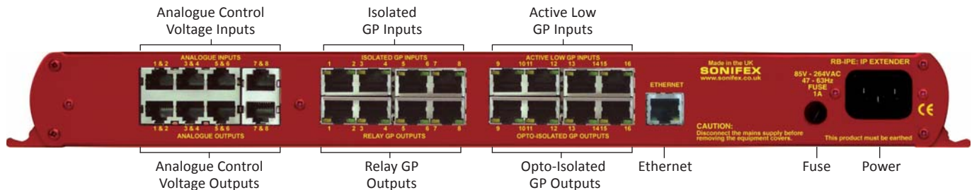
Fig 11-4: RB-IPE Rear Panel
