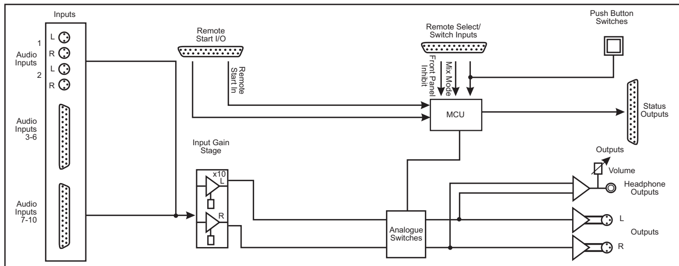
Fig 1-2: RB-SS10 System Block Diagram
