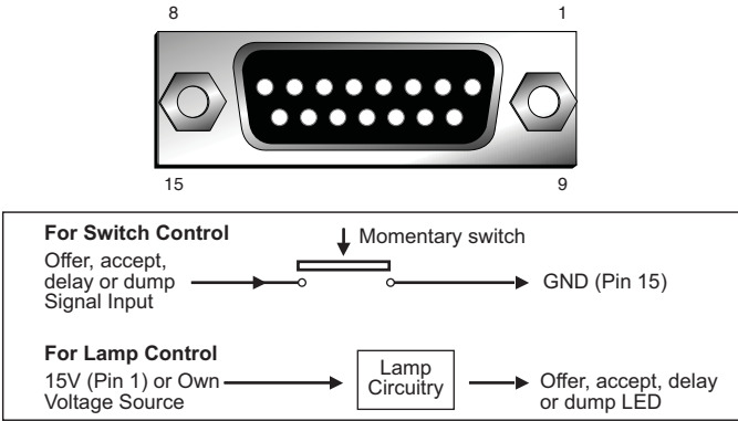
Fig 6-20: RB-OA3 Switch & Lamp Control Details
