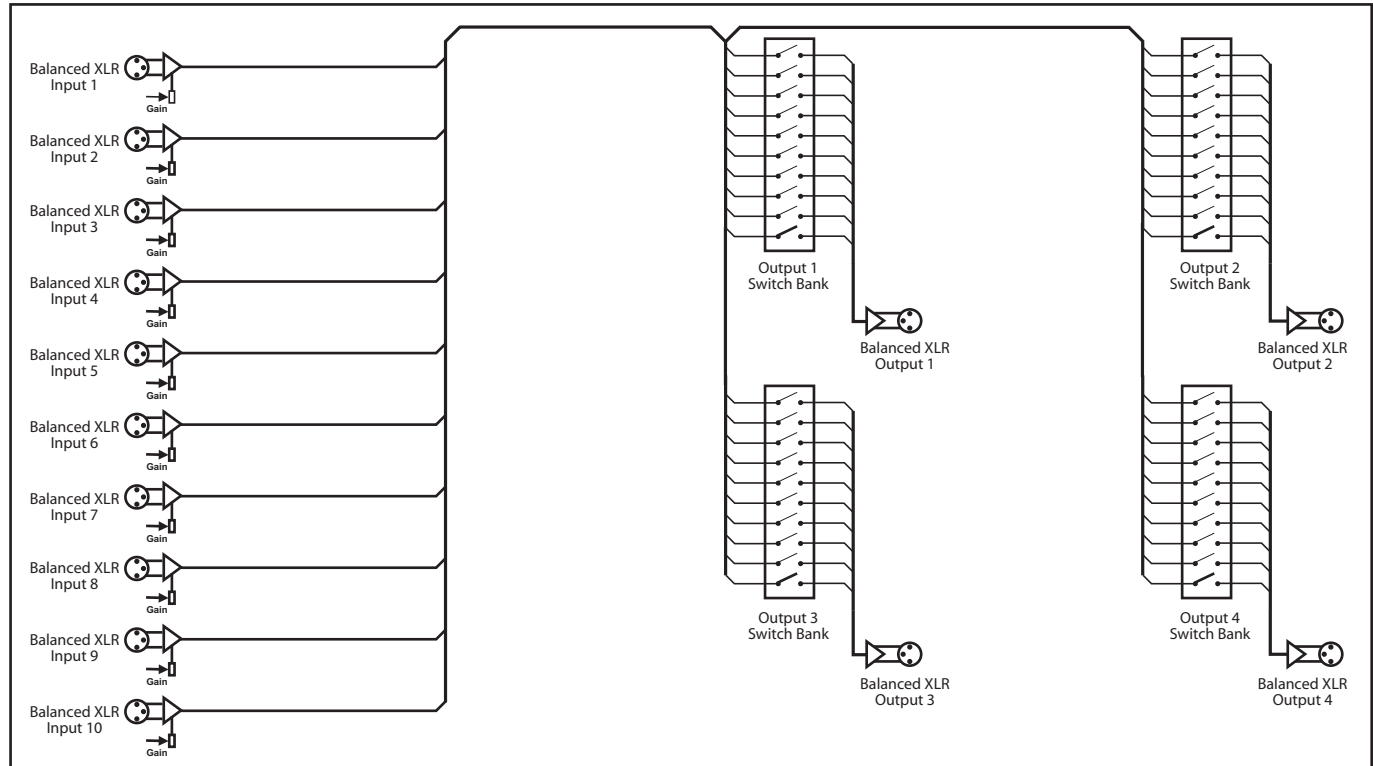
Fig 3-2: RB-PMX4 Block Diagram
