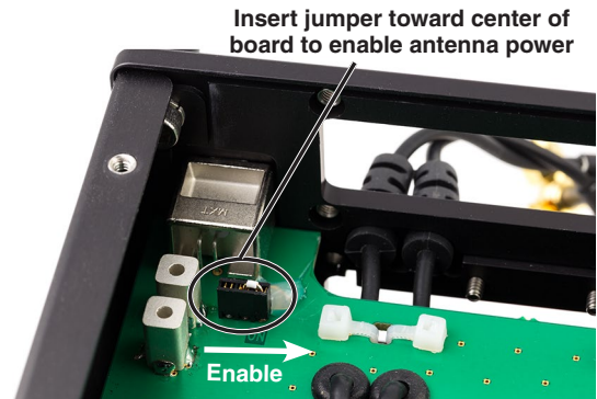
Insert jumper toward center of board to enable antenna power
