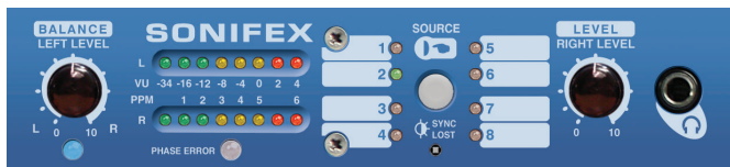
Fig 1-5: RM-CAD8 Front Panel Controls
