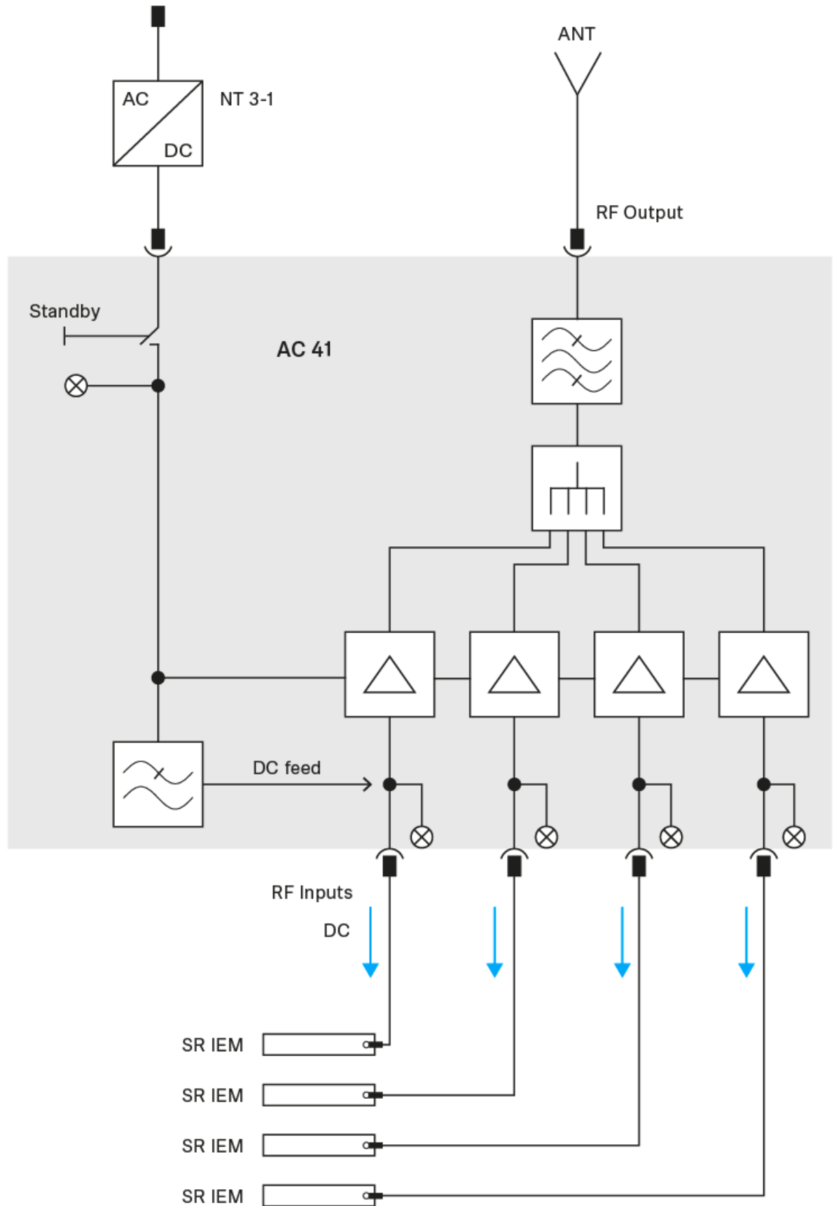
Block diagram AC 41
