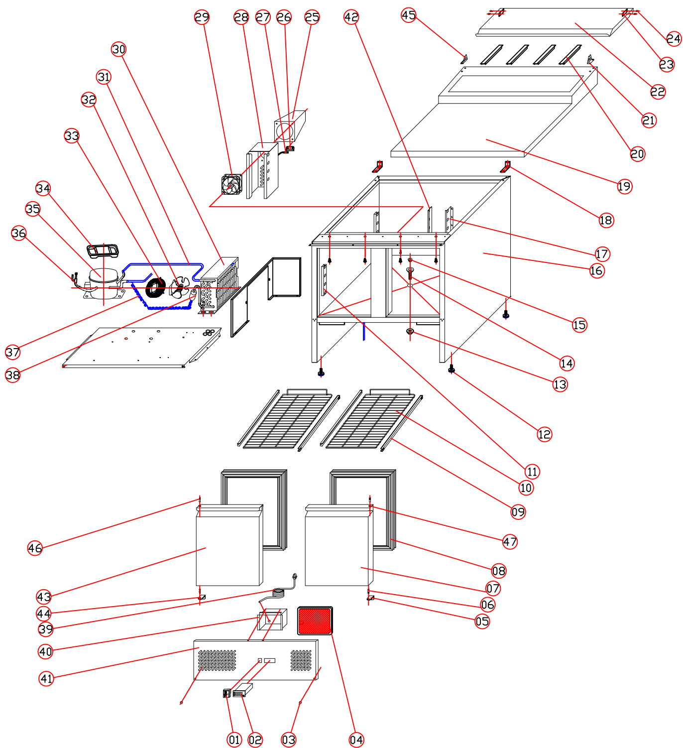
EXPLODED VIEW OF PS200GN1/6
