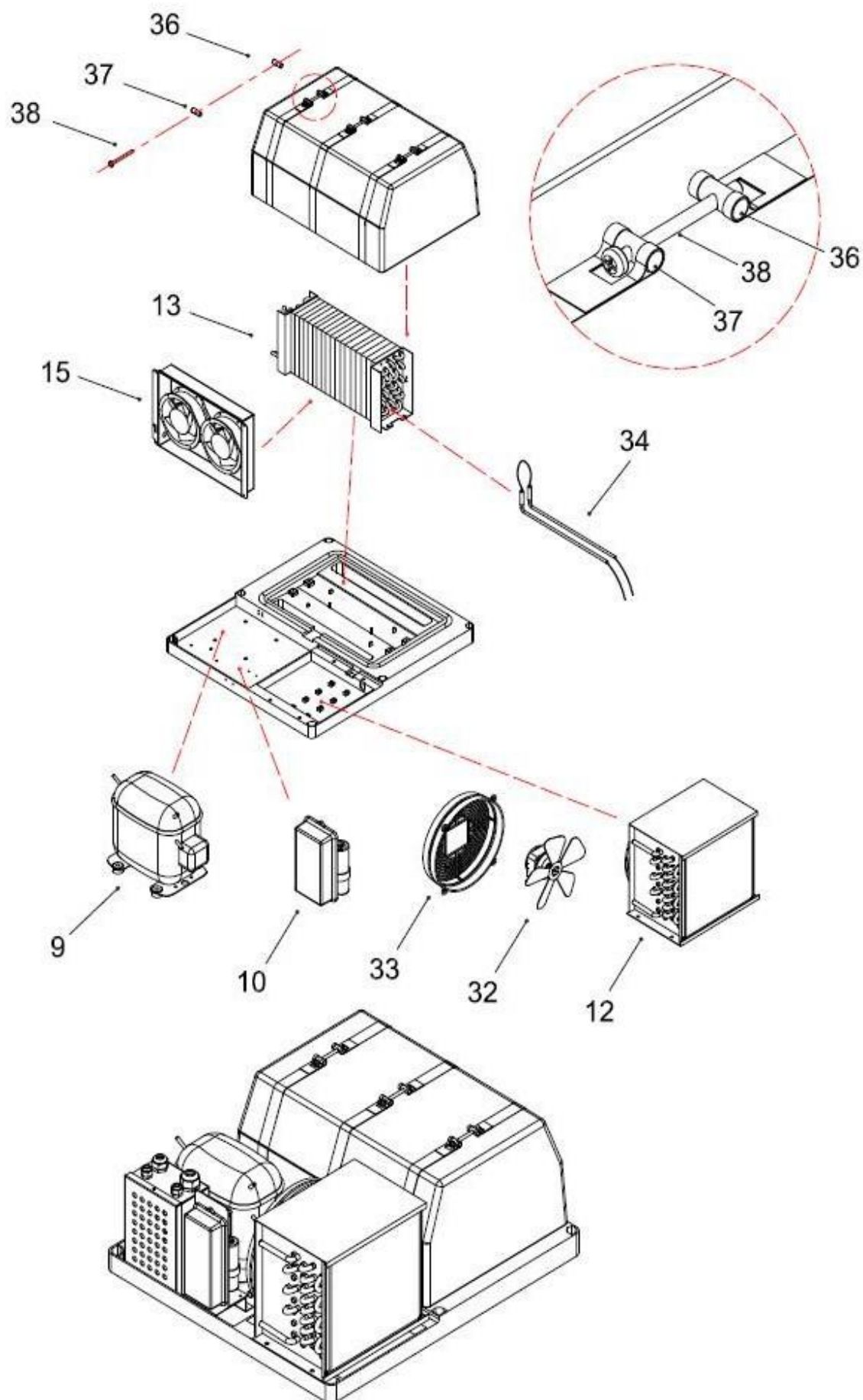
VN14-M MONOBLOCK COLLING GROUP – 01A01SG144
