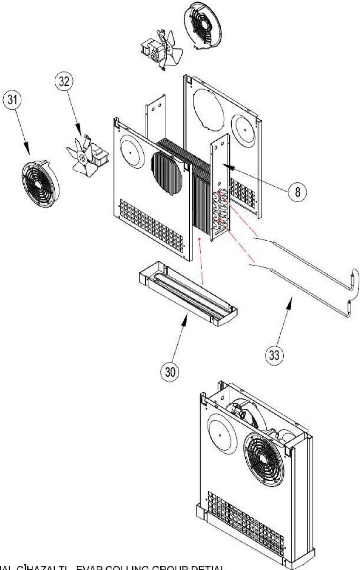
NORMAL CİHAZALTI - EVAP COLLING GROUP DETIAL
