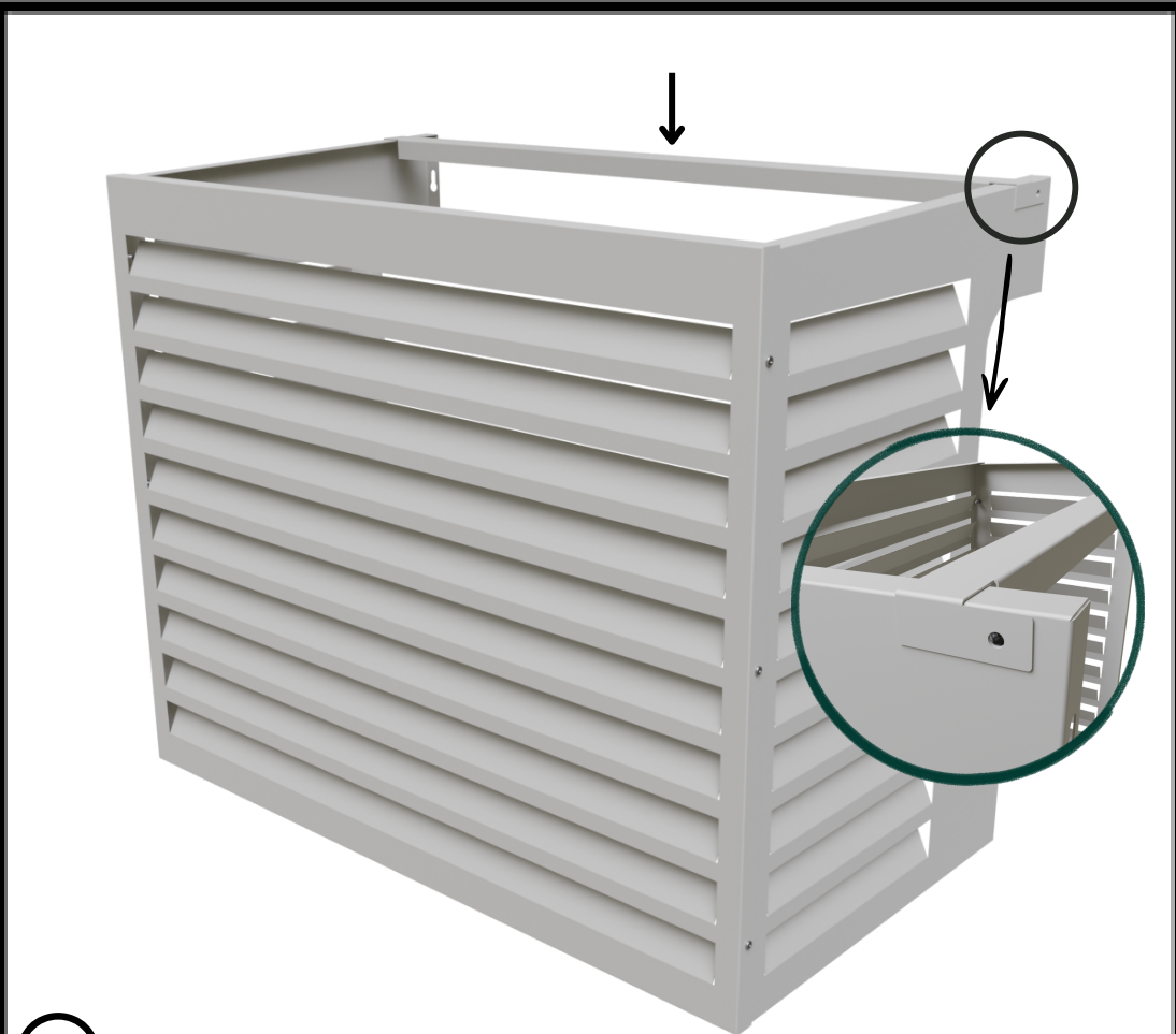
② Place the support bar.
