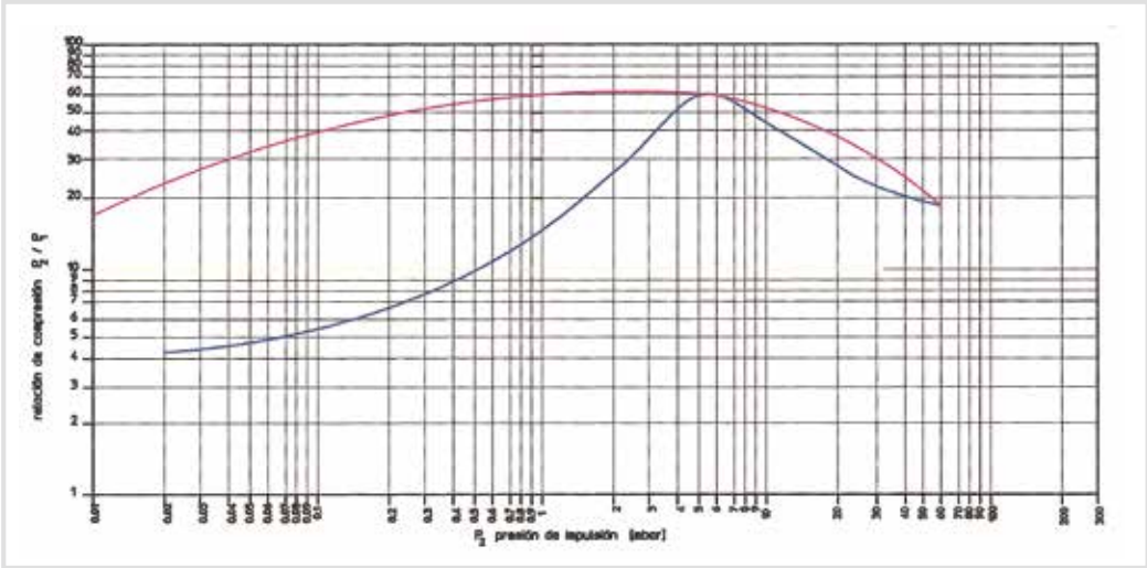
Curva acoplamiento magnético Magnetic coupling curve Curva acoplamiento convencional Conventional coupling curve
