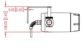
SIDE VIEW Wall Mount
