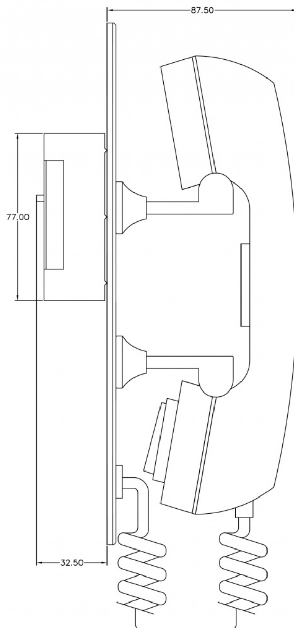
SIDE VIEW
