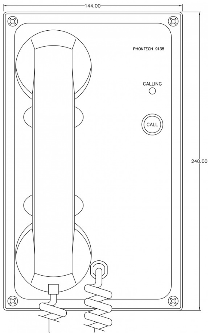
FRONT VIEW
