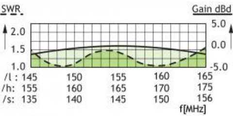
TYPICAL GAIN AND SWR CURVES
