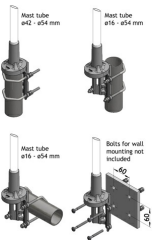
MULTI-PURPOSE MOUNTING BRACKET
