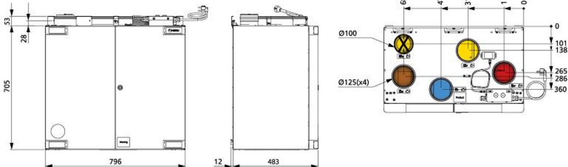
RIGHT-HAND DESIGN with cooker hood connection (mm)
