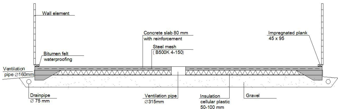
Foundation, section A - A :
