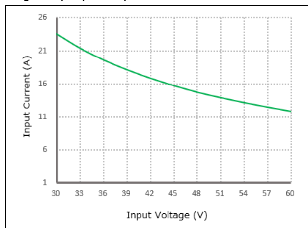
Figure 3, Input V-I, Iout=50A
