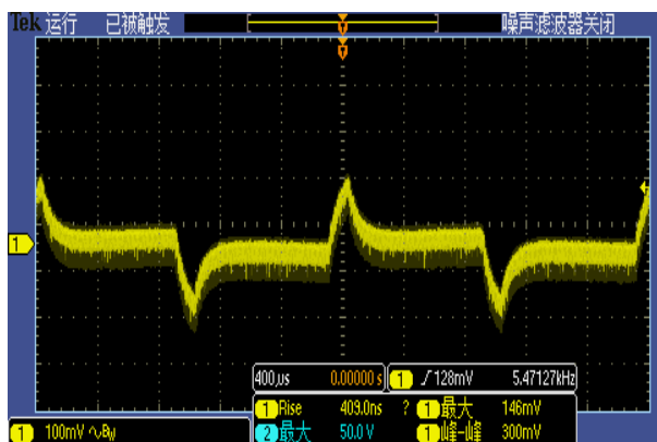
Figure 4, 25% - 50% load dynamic
