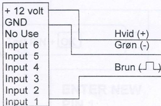
DIGMESA Flow.
