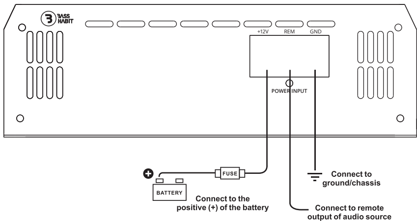
FIG 1.5: POWER CONNECTIONS FOR SE5100.1DF
