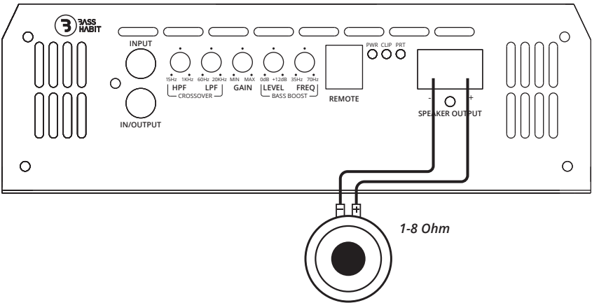
FIG 2: SPEAKER CONNECTIONS
