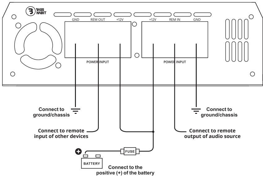
FIG 1.5: POWER CONNECTIONS FOR SE5100.1DF
