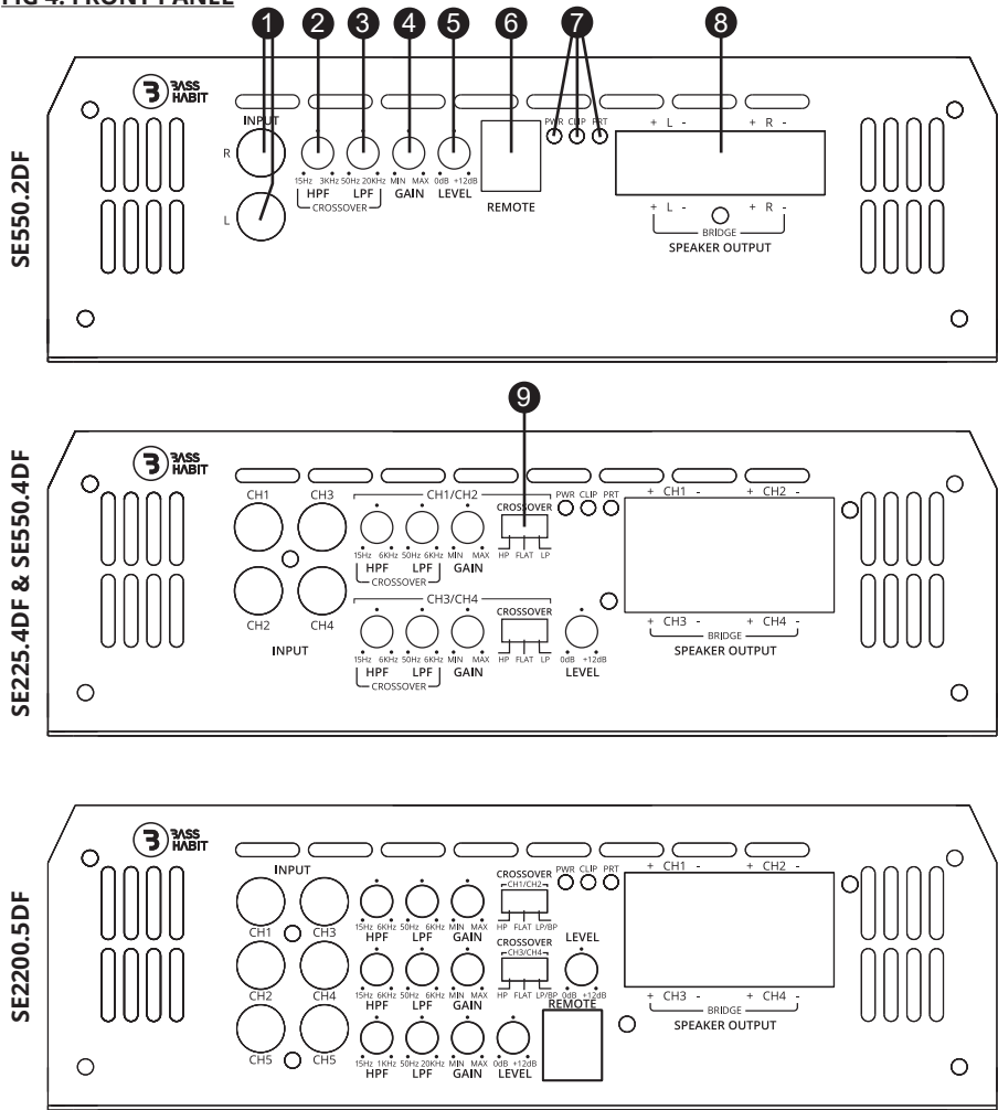
FIG 4: FRONT PANEL
