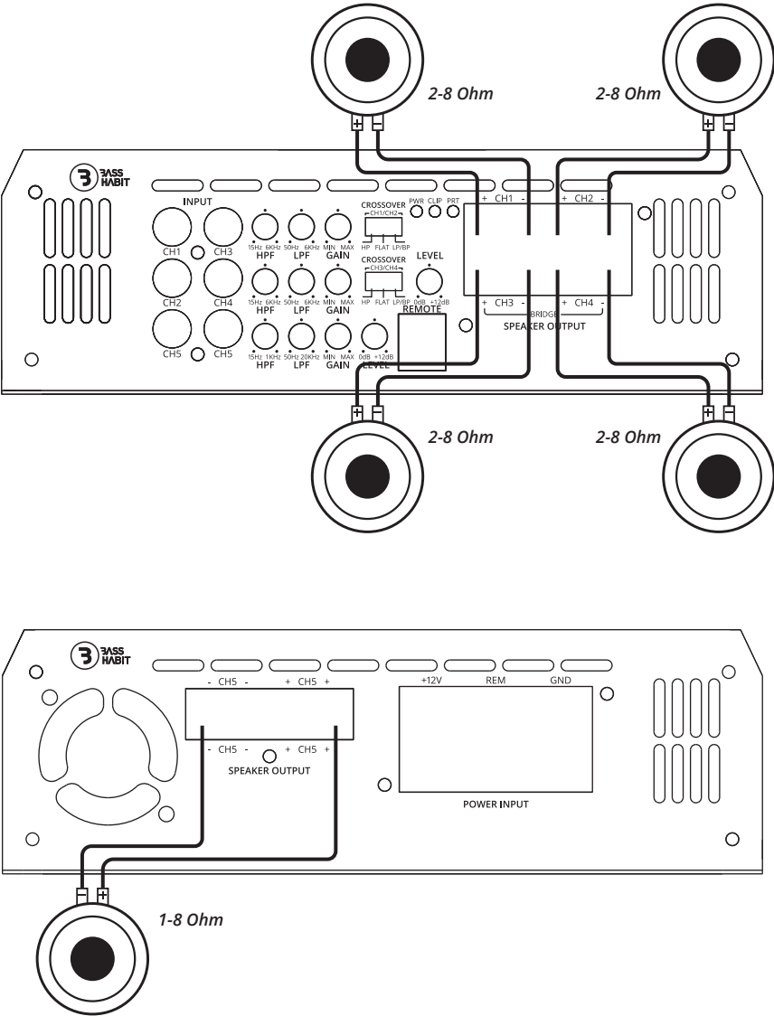
FIG 6: SPEAKER CONNECTION FIVE CHANNEL AMPLIFIER
