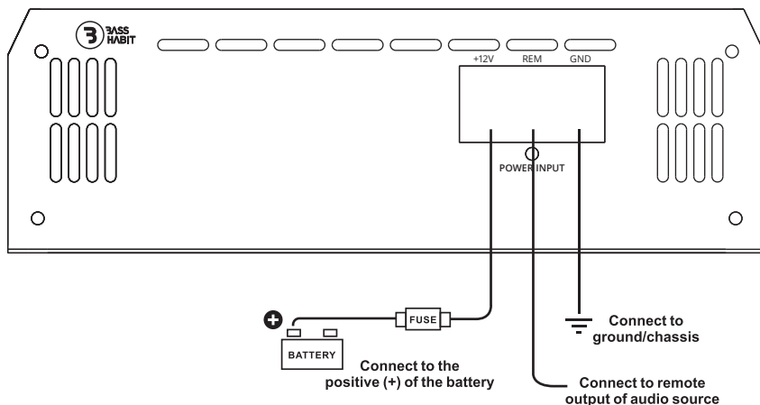
FIG 1: POWER CONNECTIONS
