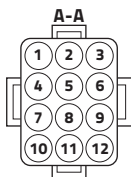
12 pin Harness pin out
