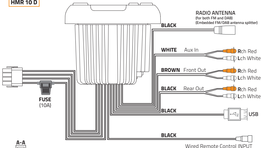
12 PIN HARNESS
