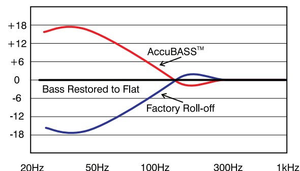
Figure 3: Shows how the AccuBASS™ operates to correct for the factory bass roll-off
