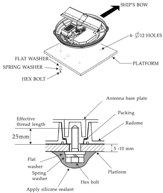
Figure 3.2.b - How to fasten the radome base to the mounting platform
