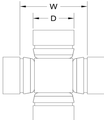
TYPE ONE INSIDE SNAP RINGS
