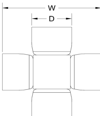
TYPE TWO OUTSIDE SNAP RINGS
