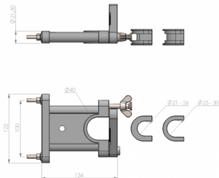
Bracket 10000-471
