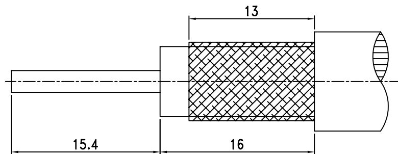
RECOMMENDED CABLE STRIPPING DIM'S (建議剝線尺寸)
