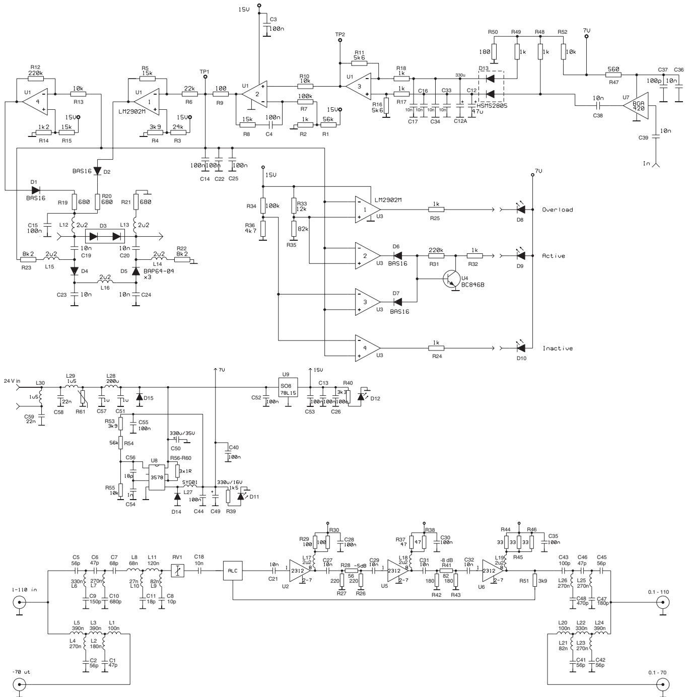
Schematic diagram for A3550/O
