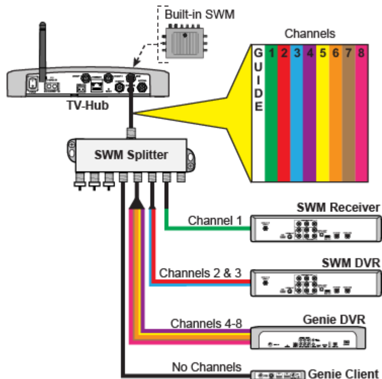
Figure 7-5 DIRECTV SWM Technology
