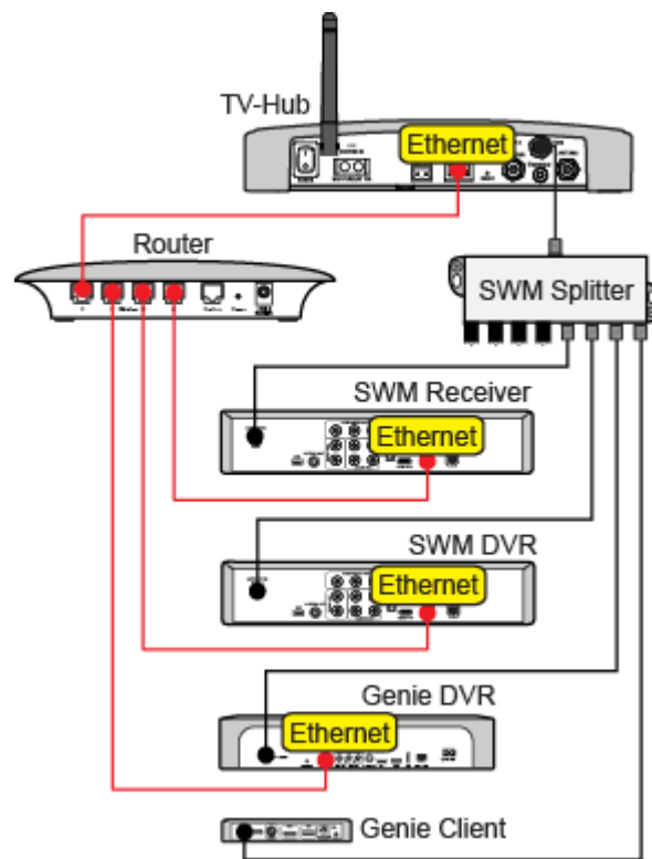
Figure 7-3 Example of Network Connections for DIRECTV
