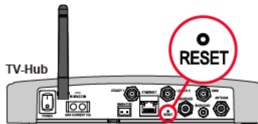
Figure 3-6 Reset Button (TV-Hub A shown)
