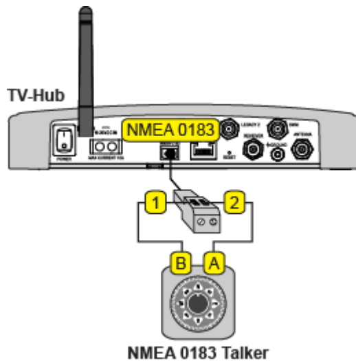
Figure 4-4 TV-Hub NMEA Connection (TV-Hub A shown)
