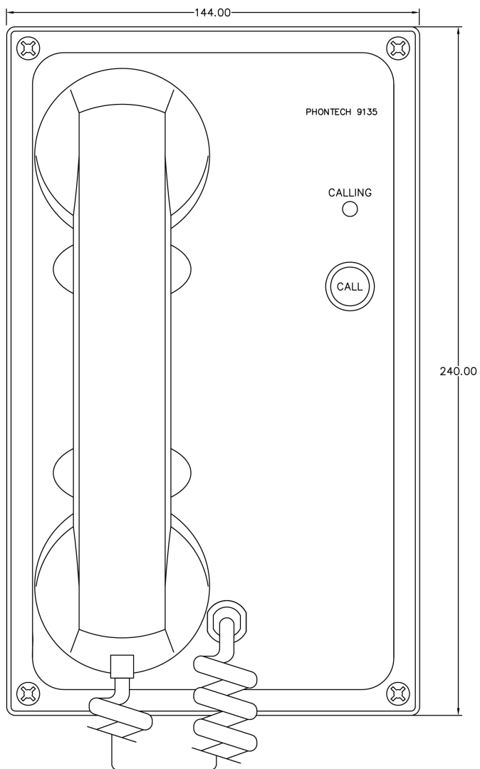
FRONT VIEW
