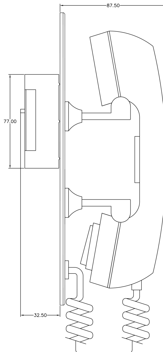
SIDE VIEW
