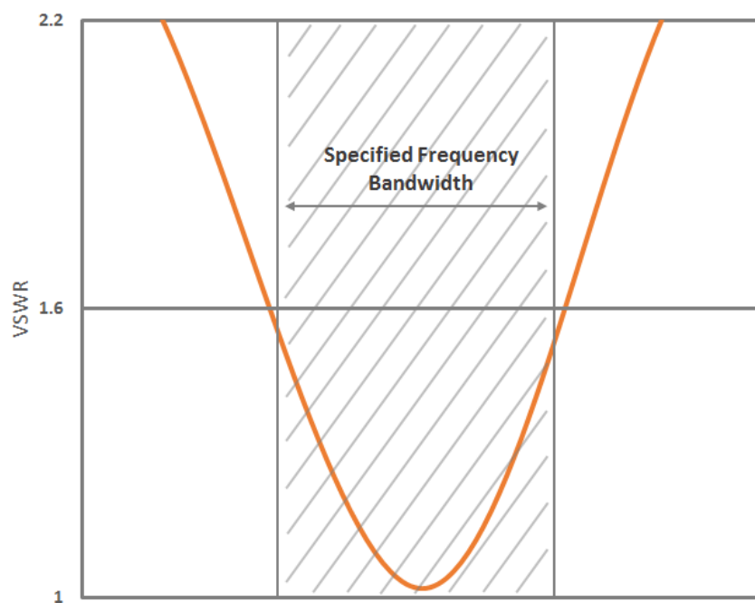
Typical VSWR
